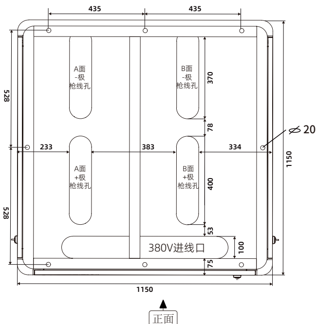
(全柔群充主机柜孔位俯视图)
