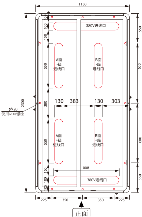
(全柔群充主机柜孔位俯视图)
