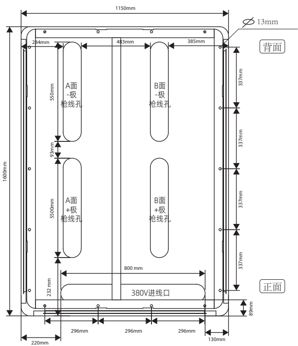
(全柔群充主机柜孔位图)
