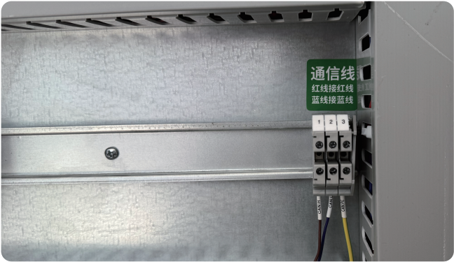
(全柔2.0群充主机柜通信CAN图)
