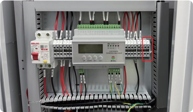
(全柔2.0群充风冷终端通信CAN图)
