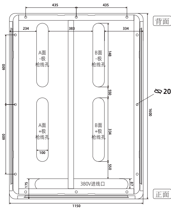
(全柔群充主机柜孔位图)
