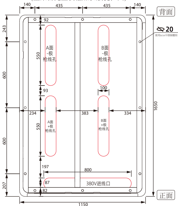
(全柔群充主机柜加长版孔位图)
